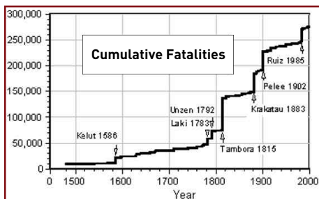
Fatal eruptions (14th century to present) and cumulative eruption fatalities (1500 to present). The overall exposure of human population to volcanic activity can be seen in the first graph, where the number of eruptions causing at least one death has steadily increased, over the last 5-6 centuries. The second graph shows that most of the lives lost during this period were lost in a few, very large eruptions. (from Simkin, Siebert and Blong, 2001)
