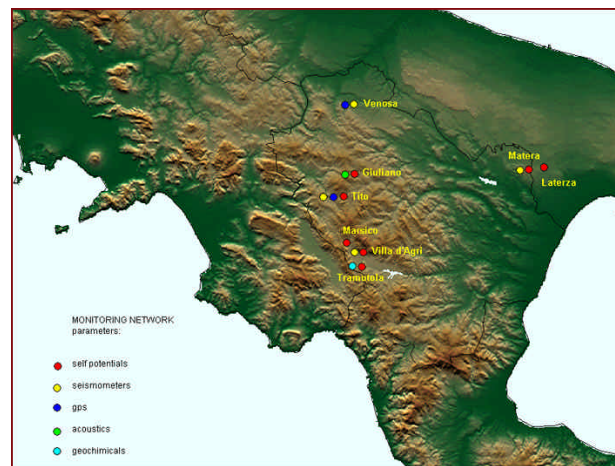
Multiparametric monitoring network installed in a seismic active area of Southern Apennine chain. The stations are equipped with sensors to detect seismometric, geodetic, geochemical and electromagnetic parameters. Contemporary plots of Self-potential, Water spring temperature, CO2 concentration, Water electrical conductivity, and Radon emission, during two months before and after an earthquake occurred in the area on April 3rd 1996 (by courtesy of IMAA-CNR).
