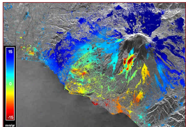
Application of the multi-interferometric technique of the Permanent Scatterers over Etna. 40 ERS scenes have been used by TRE, a spinoff company of Politecnico di Milano to create this image accounting for average deformations along satellite's line of sight occurred during the time interval 1995-2000. Faults dividing areas characterised by different deformation rates and trend are clearly visible as well as subsidence on the western part of the area. (image courtesy of TRE)
