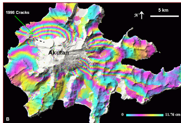
A: interferogram of Akutan Volcano in the Aleutians, made from C-band ERS imagery (Lu and others, JGR, 2000) is only locally coherent (rainbow areas). B: interferogram made from L-band JERS data (Lu and others, GRL, 2003) has fewer fringes, but achieves coherence over almost the entire surface of the island, allowing us to see the entire deformation pattern. To date, the JERS SAR mission has not been followed up with a new L-band instrument and so such observations are not currently possible. (image Courtesy of USGS)
