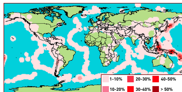
Annual probability of earthquake occurrence within 200 km with a Magnitude greater than 5.4 on Richter scale. Data source: Council of the National Seismic System (CNSS). Data analysis, mapping and printing: UNEP/GRID-Geneva, June 2000. (from http://www.grid.unep.ch/ )
