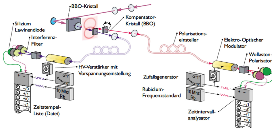
Fig. 8. Timing experiment of Zeilinger's group (Weihs et al. [52]). The EPR source is a so-called BBO crystal pumped by a laser, the outgoing photons are vertically and horizontally polarized on two different cones and in the overlap region they are entangled. These entangled photons are led separately via optical fibers to the measurement stations Alice and Bob. During the photon propagation the orientations of polarizations are changed by an electro-optic modulator which is driven by a truly random number generator, on each side. The figure is taken from reference [53], © Gregor Weihs. (This figure is subject to copyright protection and is not covered by a Creative Commons license.)
