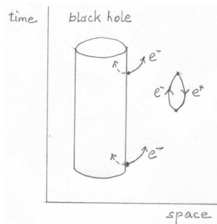
Fig. 22. Hawking radiation. The vacuum fluctuations of the quantum field, the creation of virtual particle–antiparticle pairs near the event horizon, where one particle falls into the black hole and the other one escapes, are responsible for the Hawking radiation.
