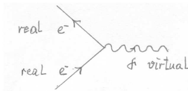
Fig. 14. Electron–photon interaction. Interaction of an electron e^- with a photon \gamma . At the vertex the two electron lines are real, the photon line is virtual.
