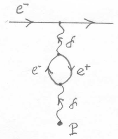
Fig. 19. Lamb shift. Shift of the levels {}^2S_{1/2} and {}^2P_{1/2} in the hydrogen atom due to the vacuum polarization of the photon.
