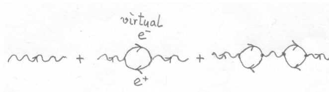
Fig. 17. Vacuum polarization of the photon. When a photon propagates it creates and annihilates permanently virtual electron e^- and positron e^+ pairs.
