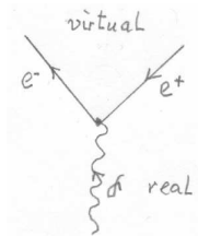
Fig. 16. Pair creation. Creation of a virtual electron e^- and positron e^+ pair from a real photon \gamma .
