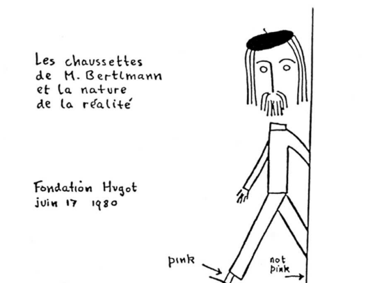
Fig. 5. Bell’s cartoon of Monsieur Bertlmann. Illustration in the CERN preprint Ref.TH.2926-CERN “ Bertlmann’s socks and the nature of reality ” of John Bell from 18th July 1980 [10]. The article is based on an invited lecture John Bell has given at le Colloque sur les “ Implications conceptuelles de la physique quantique ”, organisé par la Fondation Hugot du Collège de France, le 17 juin 1980, published in Journal de Physique [11]. (This figure is subject to copyright protection and is not covered by a Creative Commons license.)
