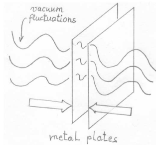
Fig. 21. Casimir effect. The vacuum fluctuations of the electromagnetic field, which are subjected to boundary conditions inside the two plates, generate a net force, either an attraction or a repulsion of the plates depending on their arrangement.
