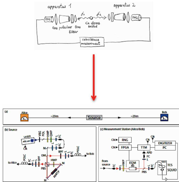
Fig. 9. Setup changes in Bell-type experiments. Above: The setup of Clauser’s experiment [41] in 1972. Below: The setup of the Zeilinger group (Giustina et al. [69]). (a) The setup of the experiment with the spatially separated measurement stations Alice and Bob. (b) The source: As a source a type-II spontaneous parametric down-conversion in a periodically poled crystal (ppKTP) is used. (c) Measurements stations: In each station Alice/Bob, one of the two linear polarization directions is selected, as controlled by an electro-optical modulator (EOM), which acts as a switchable polarization rotator in front of a PBS plate. The signals are amplified and recorded together with the setting choices. The figure is taken from Giustina et al. [69], © Anton Zeilinger.
