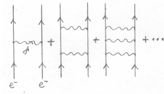
Fig. 18. Electron–electron scattering. In the interaction of two electrons one virtual photon is exchanged to lowest order of approximation, two photons are exchanged to the next order, three photons next etc.
