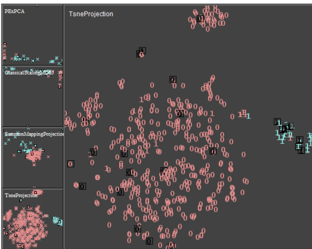
Figure 4: Visual observation of the FRAUD dataset after 25 iterations using a class-based color coding. Frauds (1-labels) build a separate cluster with all dimensionality reduction techniques. In t-SNE it can be seen that few fraud instances in the large 0 cluster are still classified as no fraud requiring individual treatment (fine tuning). After iteration 10 the average F1 score remained at about 0.96. F1 was chosen to account for the unbalanced class priors.
