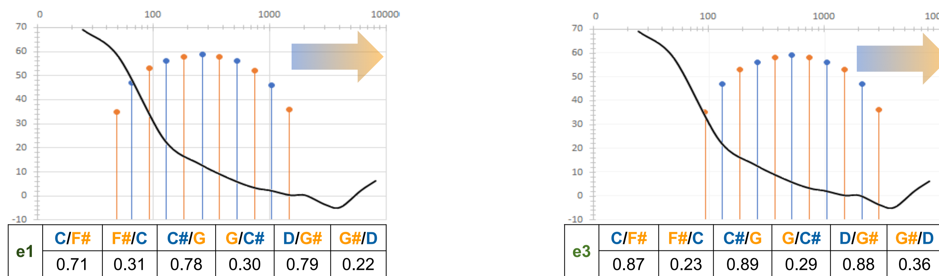
Fig. 2: Amplitudes and frequencies of the tritone interval C-F# below the envelopes e1 and e3. Table: Mean values of the participants' judgments for C-F#, C#-G and D-G# (1 = the interval rises, 0 = the interval falls). The direction of movement of partials 1-6 (especially the higher ones) determines the perceived interval direction.
