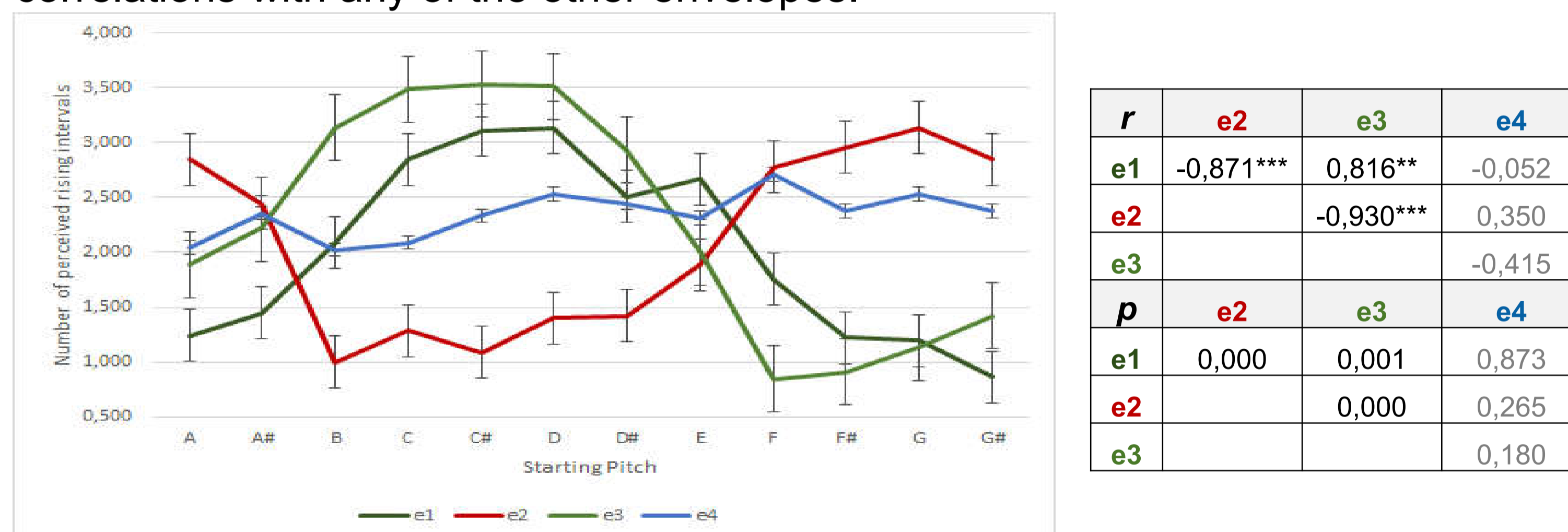
Fig. 4: Perceived interval direction for stimuli with e1, e2, e3, and e4 envelopes. Table: Results of a correlation analysis on the perceived interval direction of Shepard tones under the envelopes e1-e4.
