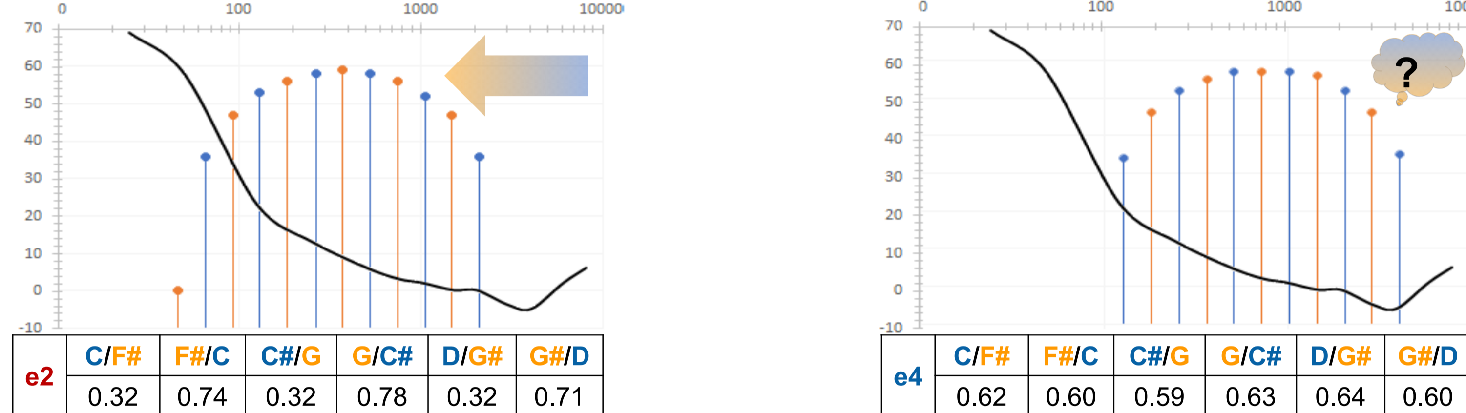
Fig. 3: Amplitudes and frequencies of the tritone intervals C-F# below the envelopes e2 and e4. Table: Mean values of the participants' judgments for C-F#, C#-G and D-G# (1 = the interval rises, 0 = the interval falls). Again, in the case of envelope e2 the direction of movement of partials 1-6 (especially the higher ones) determines the perceived interval direction. However, this does not apply to the stimuli under envelope e4.
