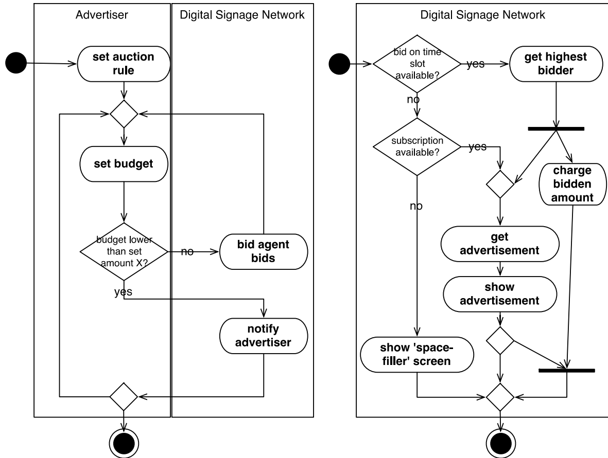
Figure 3. UML activity diagram for an exemplary rule set and backend services
