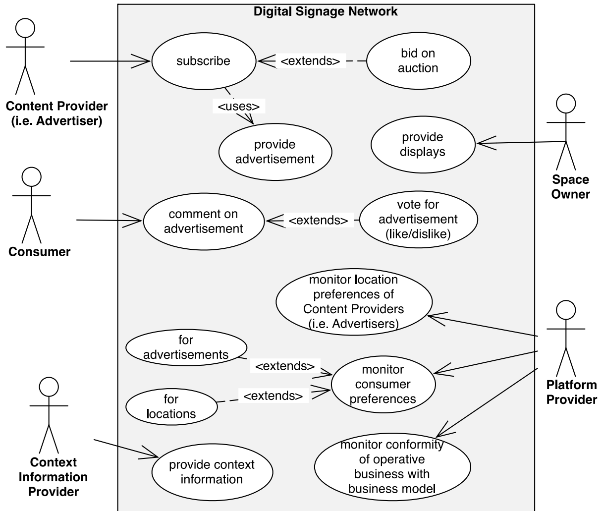
Figure 4. Exemplary UML use case diagram, displaying market players, their activities and backend services
