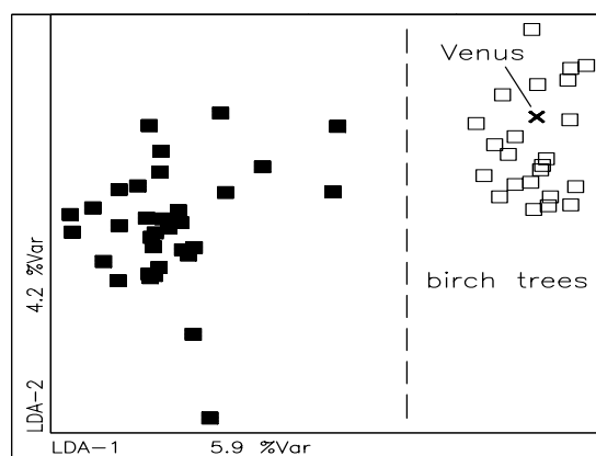
Figure 5: Linear discriminant analysis separates birch trees from other trees: the archaeological sample (x) can be definitely assigned to the betula group.
