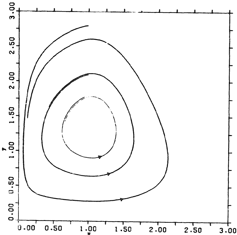
FIG. 1. Phase portrait of (1) with s = 1.05 and c, g(x), p(x) as above. The inner and outer solution, starting at (1.18) and (1.28) , respectively, spiral inwards; the middle solution with initial point (1.2099) spirals outwards. This shows the existence of two limit cycles, an unstable one lying inside a stable one.
