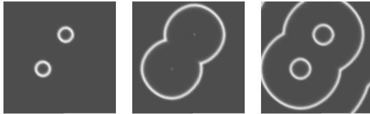
Fig. 3. Time sequence of cAMP waves on a square domain.
