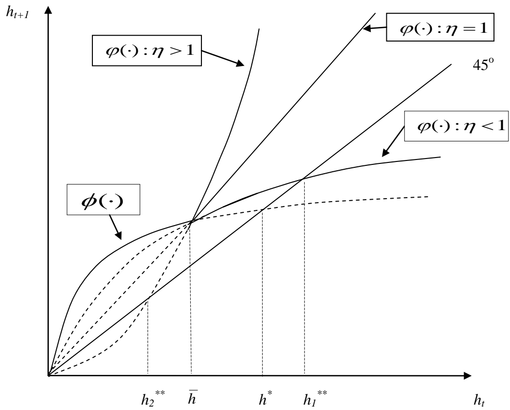
Figure 3: The phase diagram of the human capital dynamics in the benchmark economy (when \bar{h} < (\alpha A / R)^{\alpha / (1 - \alpha - \beta)} )
