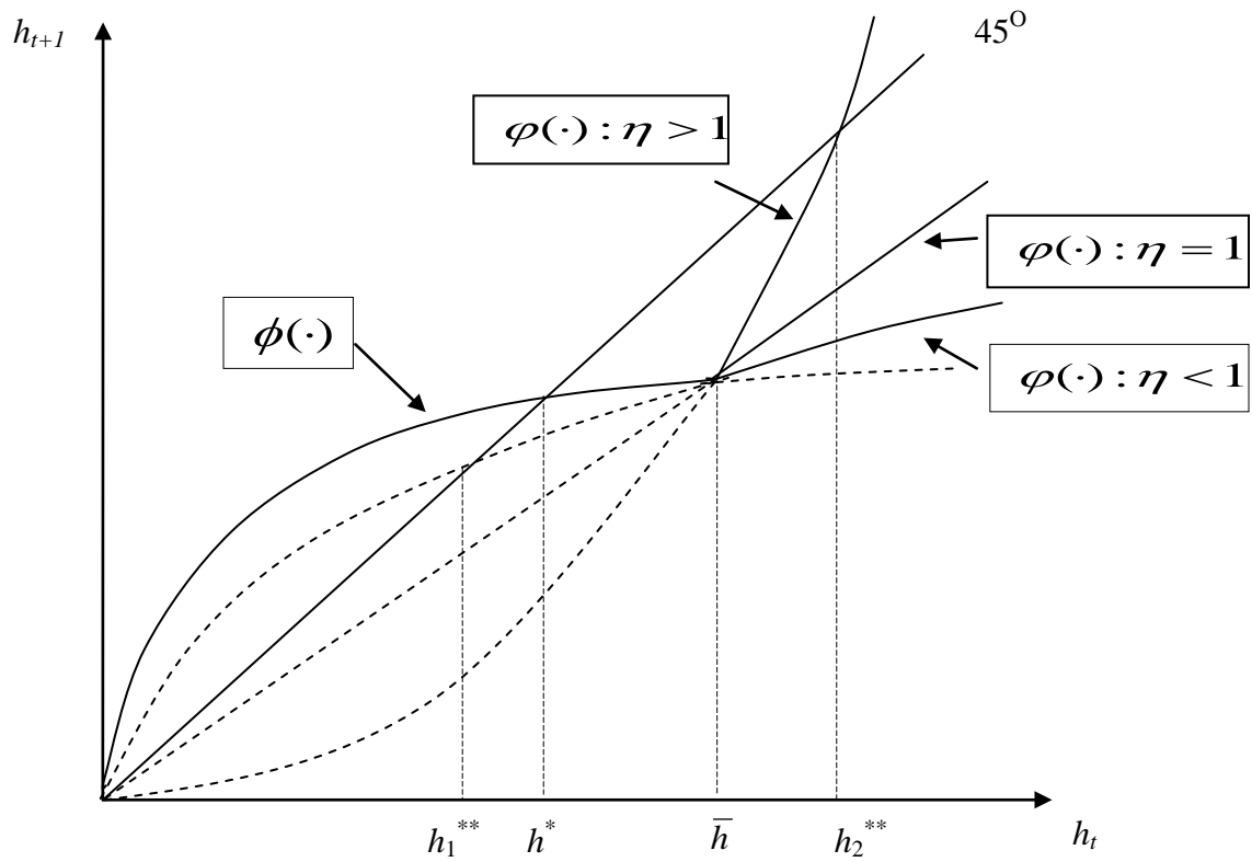
Figure 1: The phase diagram of the human capital dynamics in the benchmark economy (when \bar{h} > (\alpha A / R)^{\alpha / (1-\alpha-\beta)} )
