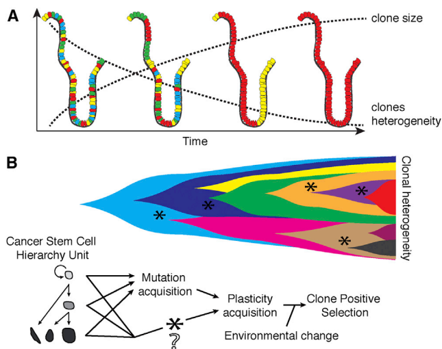
Figure 3. Clonal Heterogeneity in Homeostasis and Cancer
