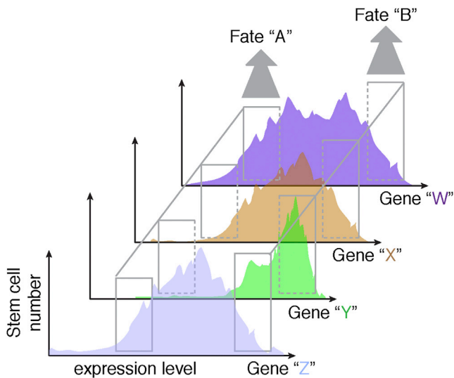
Figure 7. Transcriptional Noise as an Epithelial Stem Cell Fate Regulator
