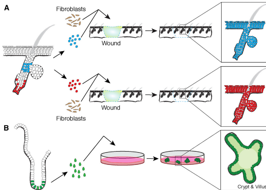
Figure 4. Stem Cell Plasticity in Tissue Reconstitution Assays
