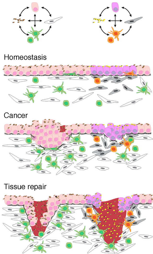
Figure 6. Fibroblasts, Immune Cells, and Bacteria as Components of the Epithelial Stem Cell Niche during Homeostasis, Tissue Repair, and Cancer
