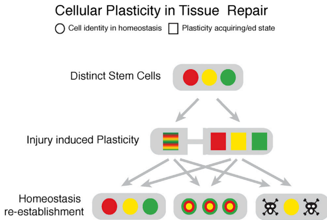
Figure 5. Model of Stem Cell Plasticity during Repair of Injured Tissue
