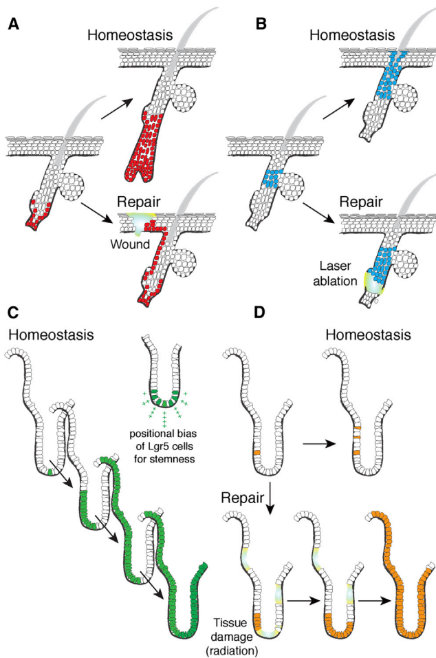
Figure 2. Epithelial Stem Cell Contributions during Tissue Homeostasis and Repair
