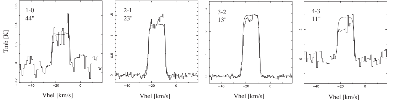
Fig. 2. SW Vir CO ( J = 1 \rightarrow 0 and 2 \rightarrow 1 ) spectra obtained with the SEST, and CO ( J = 3 \rightarrow 2 and 4 \rightarrow 3 ) spectra obtained with the JCMT (histograms). The line profiles from the best-fit model are shown as solid, thin lines (the beam size is given in each panel).
